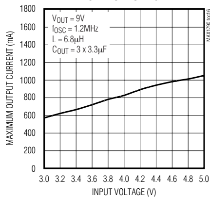
MAX8715 MAXIMUM OUTPUT CURRENT vs. INPUT VOLTAGE
