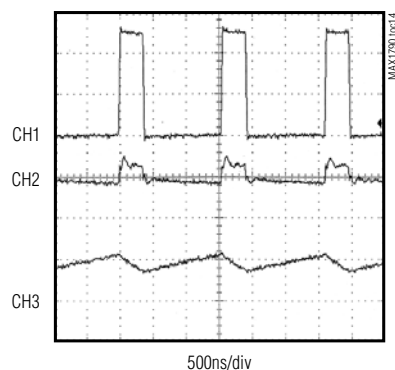
SWITCHING WAVEFORM
